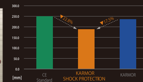
Top Primary Shock Free Fall Height
