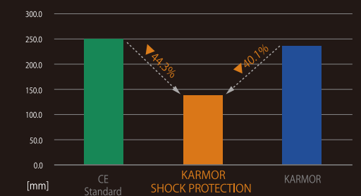
Top Secondary Shock Free Fall Height
